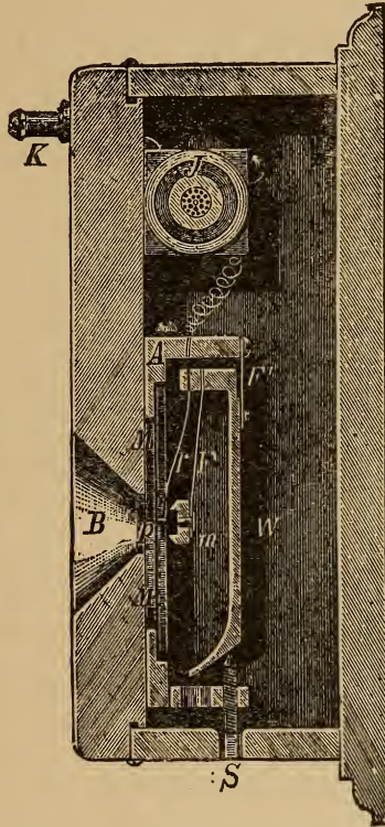
Fig. 31. BLAKE'S TRANSMITTER.
